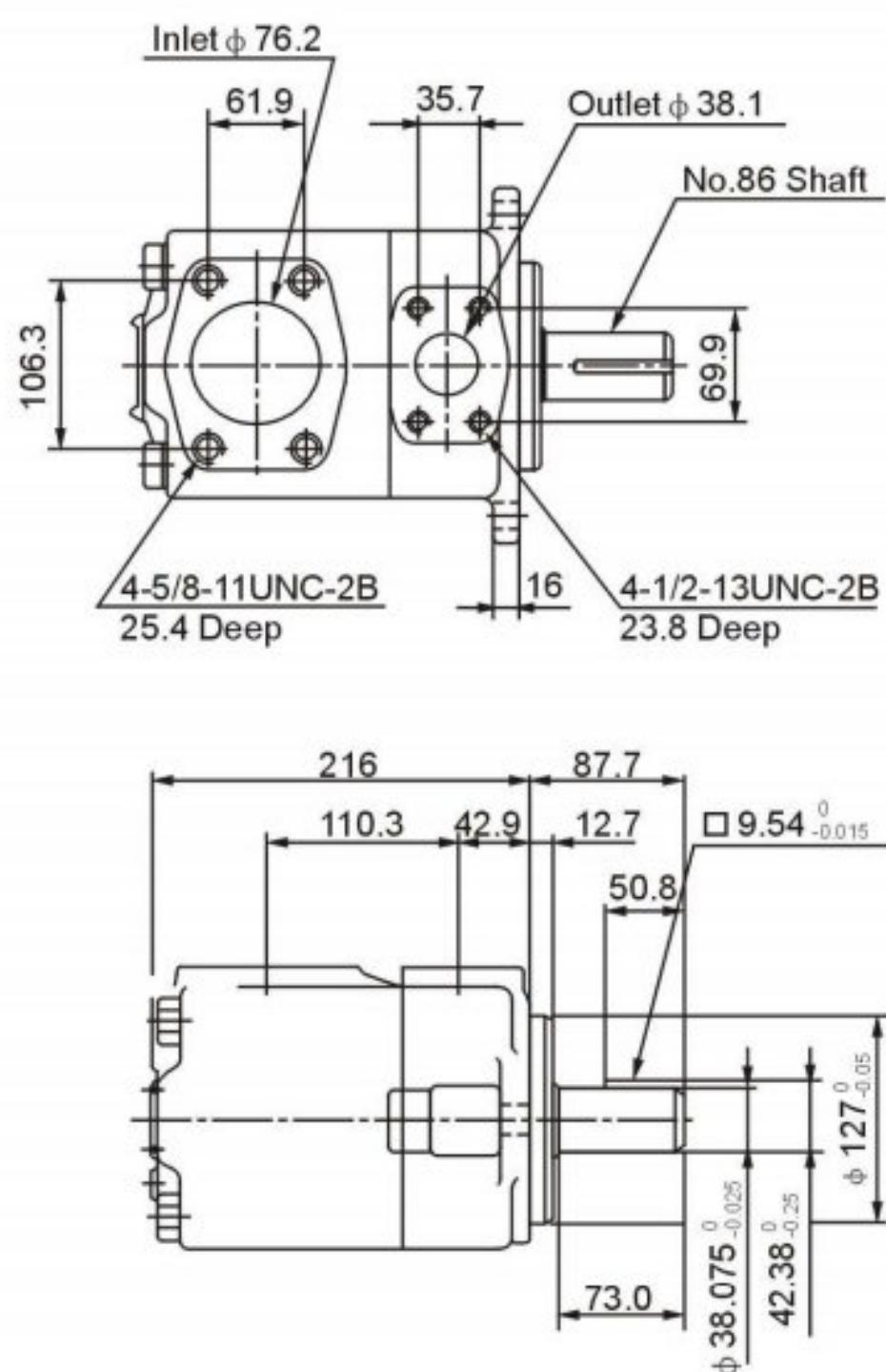
45VQ Flange Mounting
