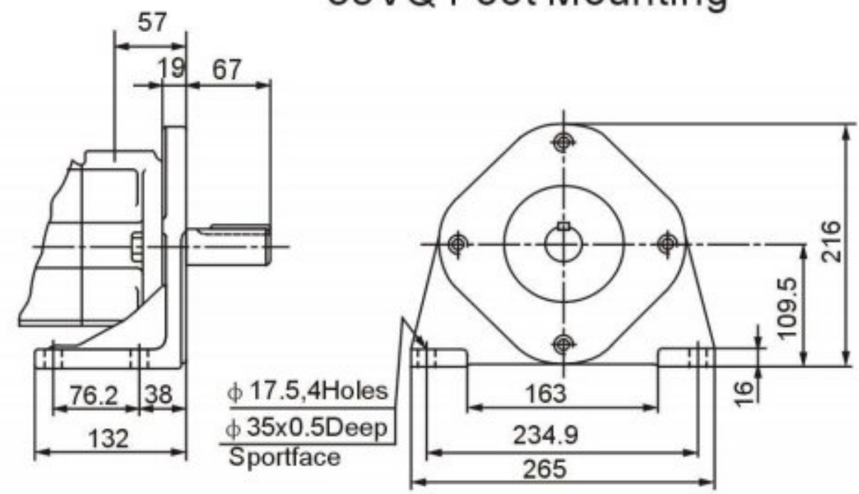
35VQ Foot Mounting
