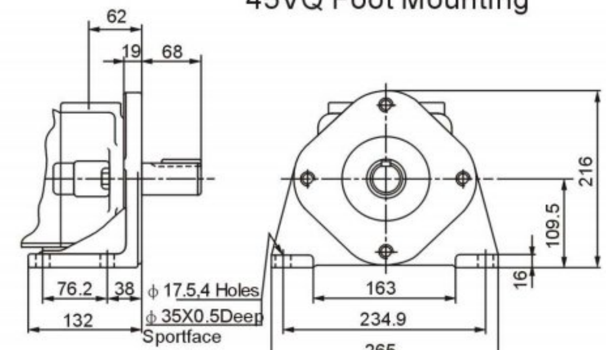
45VQ Foot Mounting
