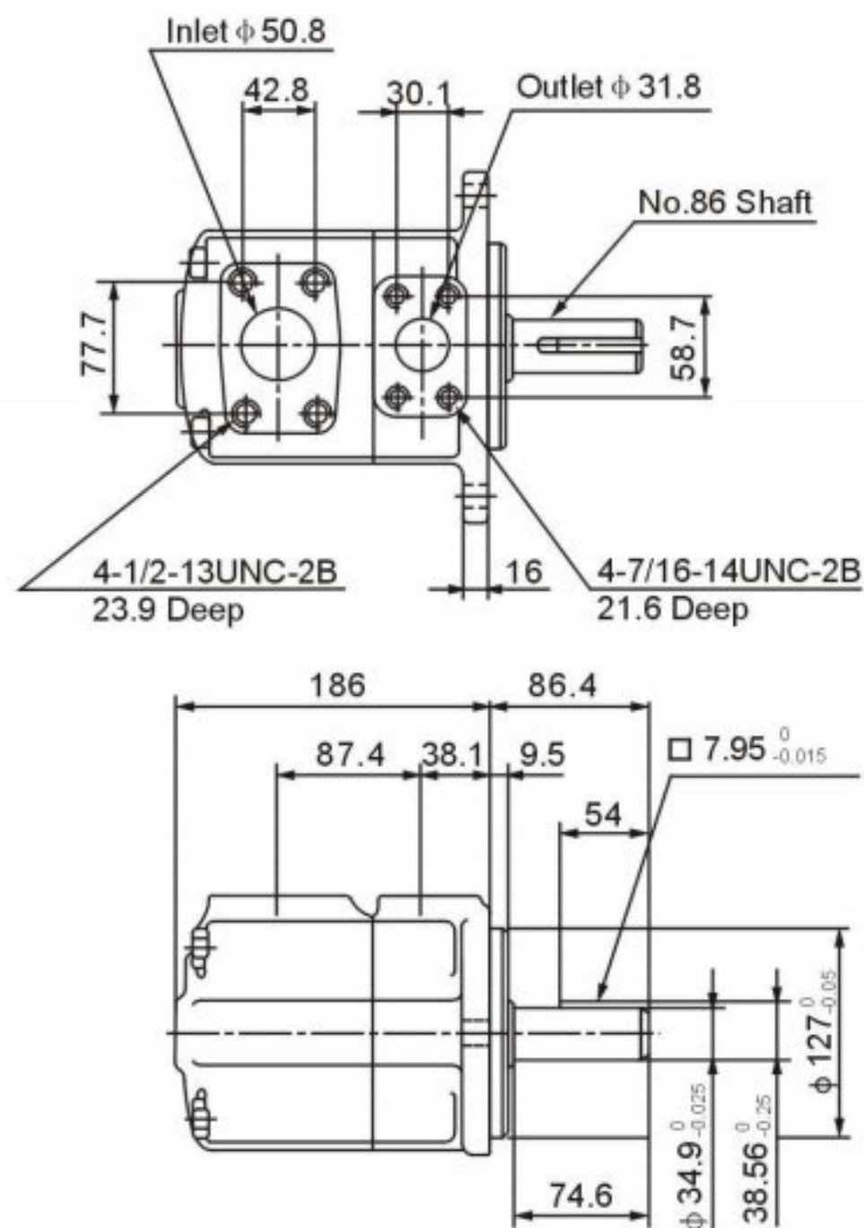
35VQ Flange Mounting
